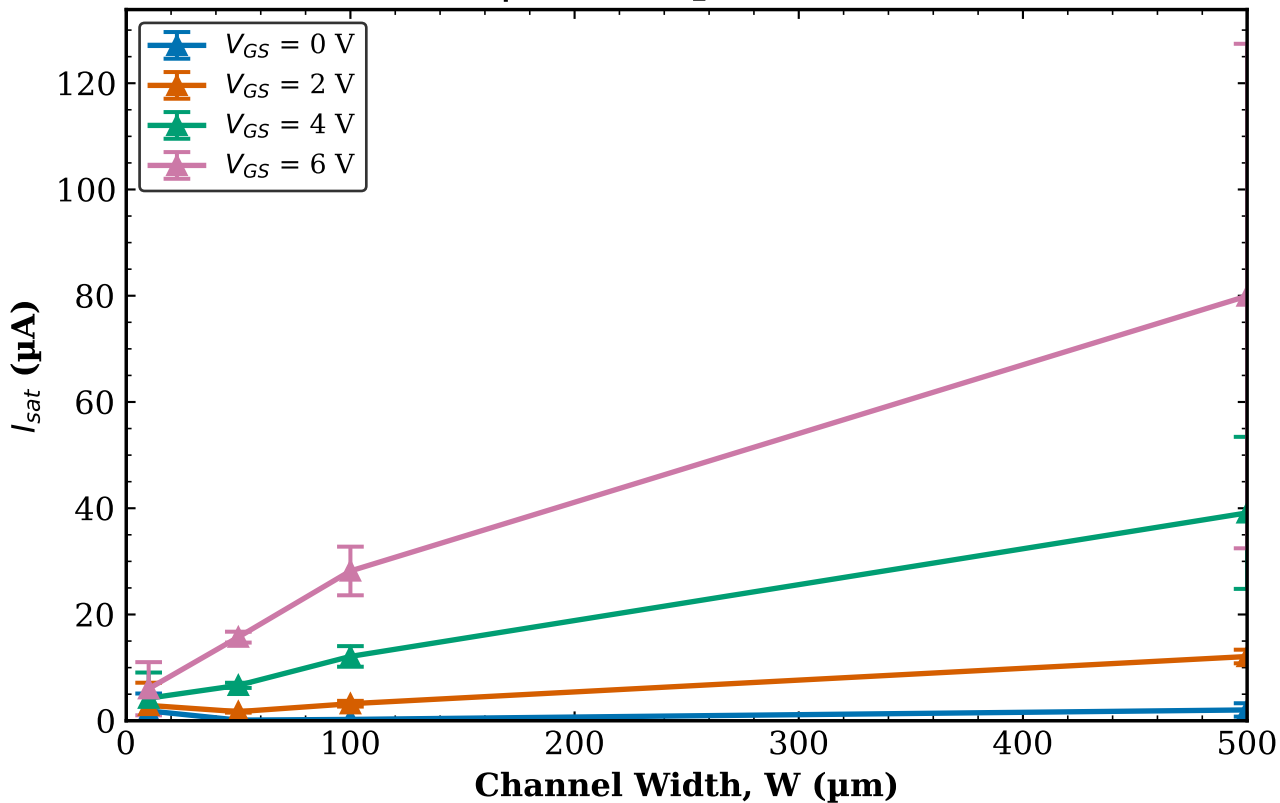
All Chips - Combined I_{sat} vs W | L = 40\text{ }\mu\text{m} (mean \pm std)
